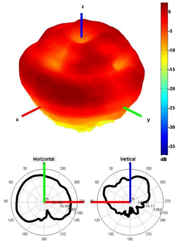
2450 and 5500 MHz Radiation pattern
